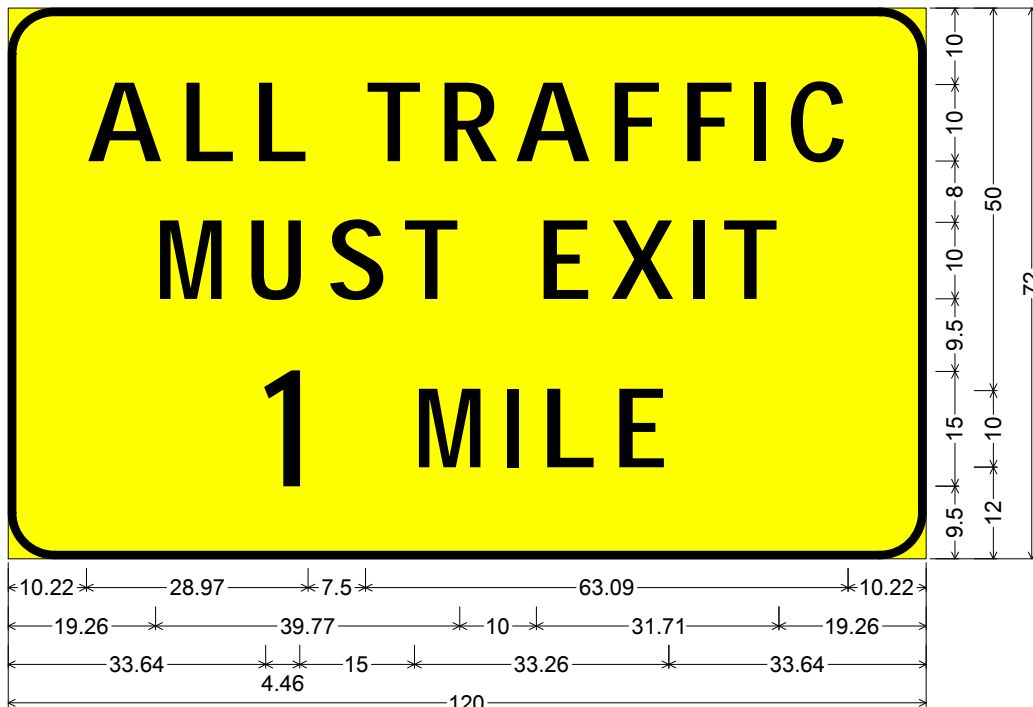
W19-05a(120x72-STD)YLW; 6.00" Radius, 1.00" Border, Black on Yellow; "ALL TRAFFIC" E Mod; "MUST EXIT" E Mod; "1" E Mod; "MILE" E Mod;
