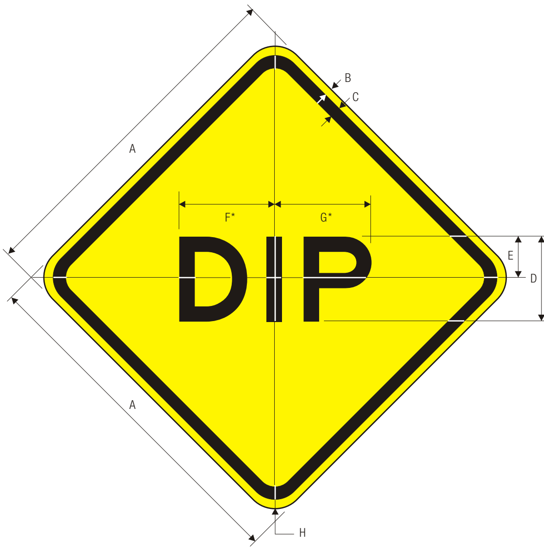
W8-2 DIP
