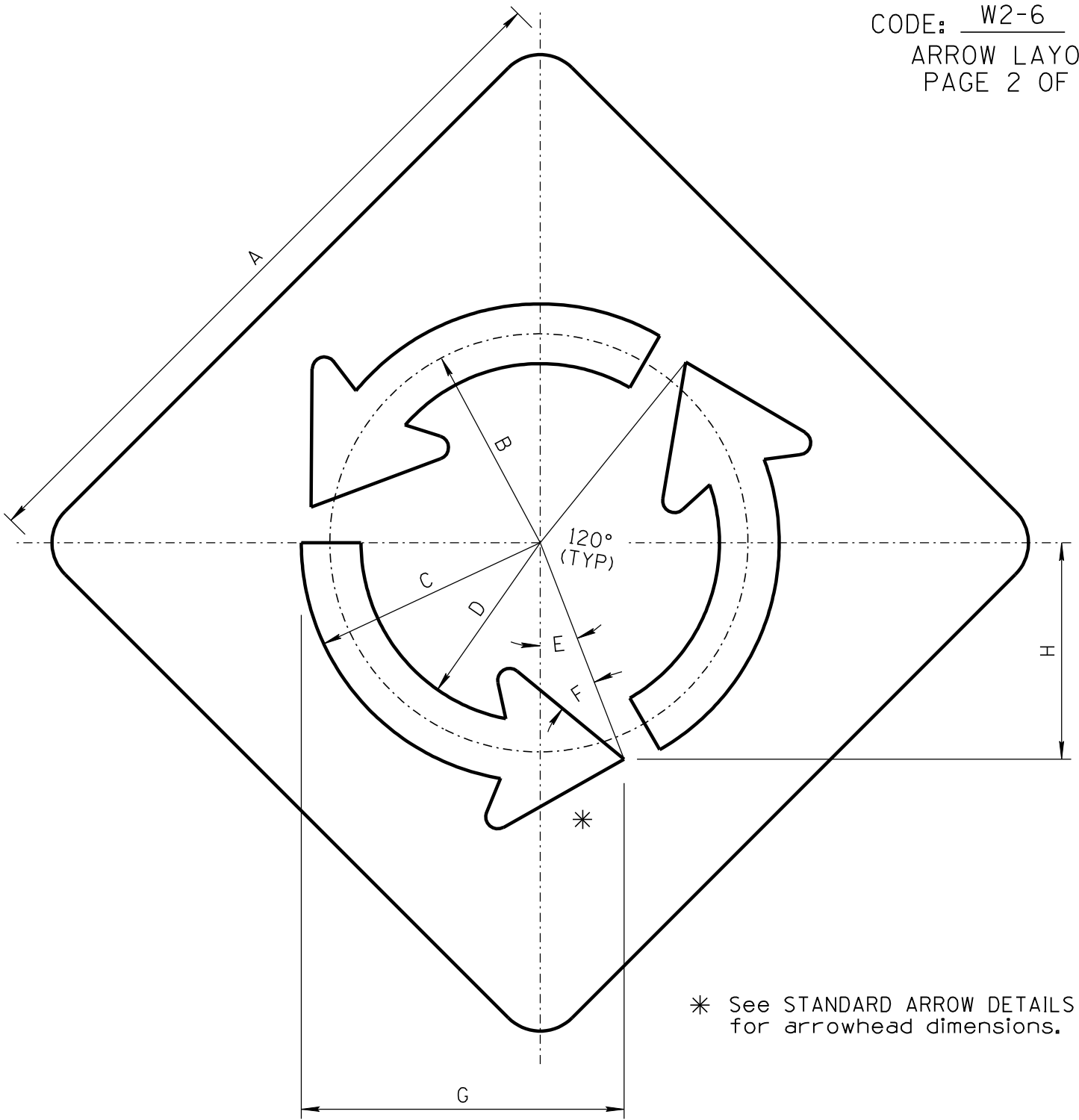
W2-6 ARROW LAYOUT BORDER AND INDENT NOT SHOWN
