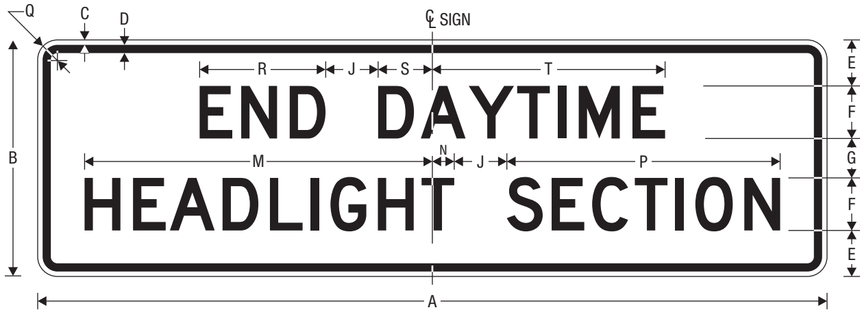
R16-11 END DAYTIME HEADLIGHT SECTION
