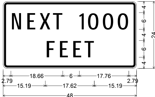
R101-003P(48x24-FWY-1000); 1.50" Radius, 0.63" Border, 0.38" Indent, Black on White; "NEXT 1000" D; "FEET" D;
