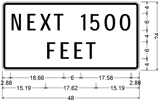
R101-003P(48x24-FWY-1500); 1.50" Radius, 0.63" Border, 0.38" Indent, Black on White; "NEXT 1500" D; "FEET" D;
