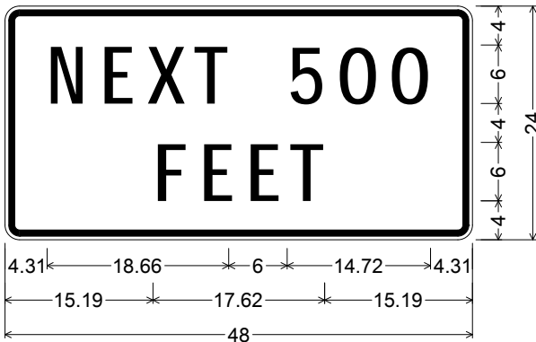
R101-003P(48x24-FWY-500); 1.50" Radius, 0.63" Border, 0.38" Indent, Black on White; "NEXT 500" D; "FEET" D;
