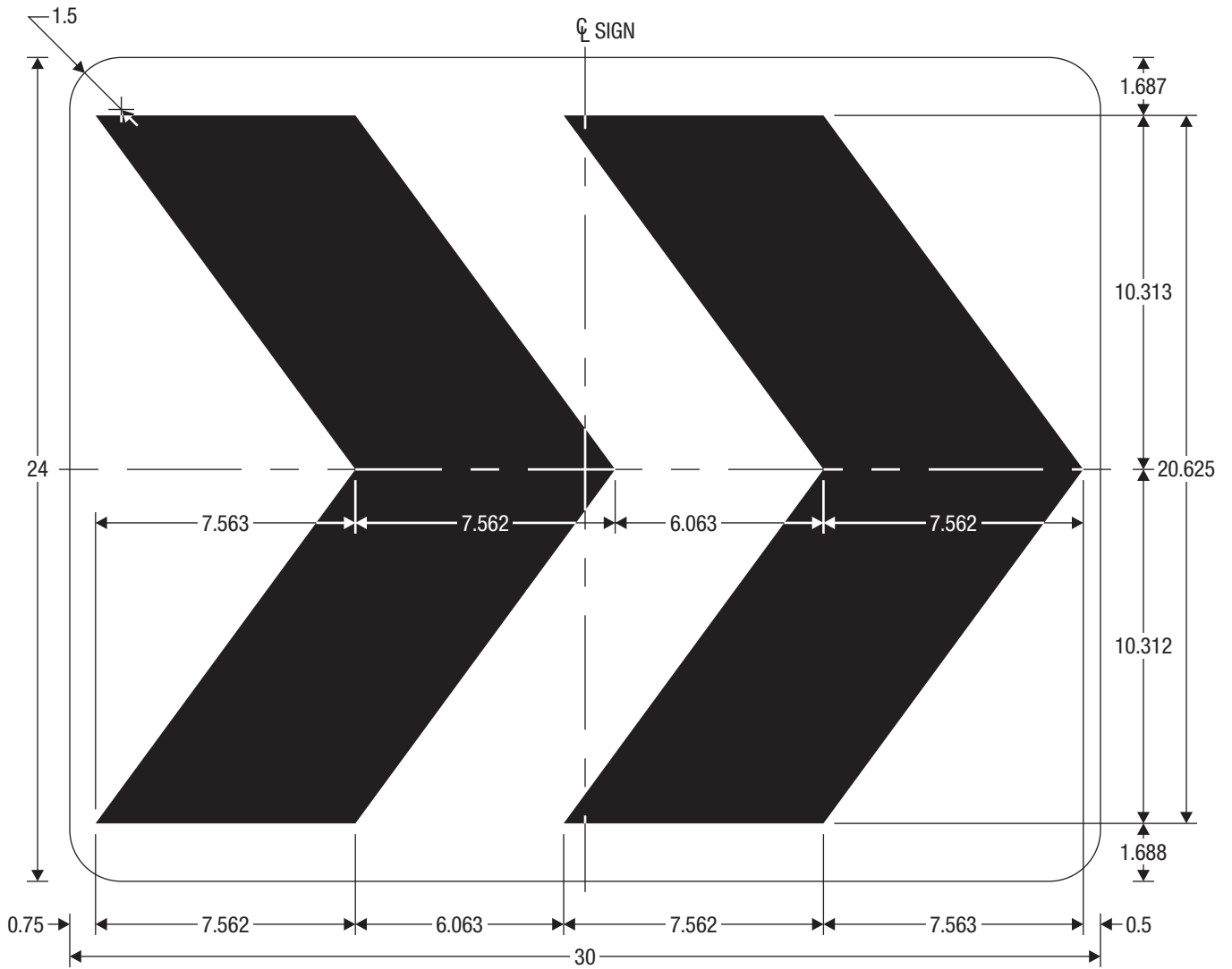
R6-4 ROUNABOUT DIRECTIONAL (2 CHEVRONS)
