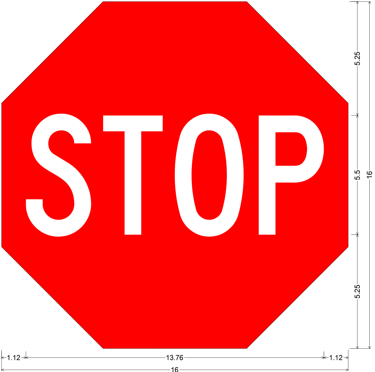
R1-1 (for use on R1-5c); No border, Red; "STOP" White C 60% spacing;
