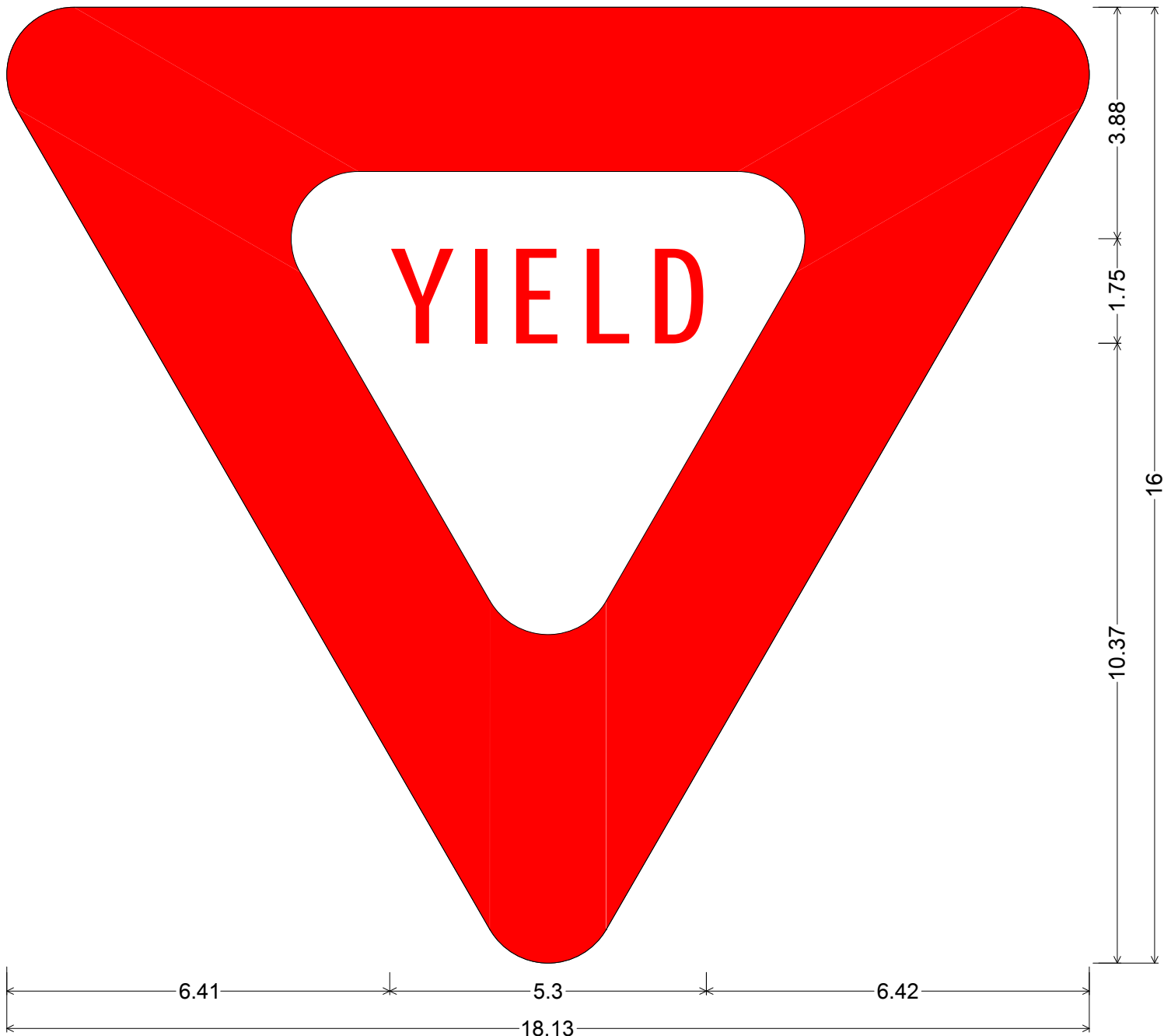
R1-2 (for use on R1-5a); 19.77" corner to corner 1.13" Radius, 2.75" Border, Red on White; "YIELD" C;
