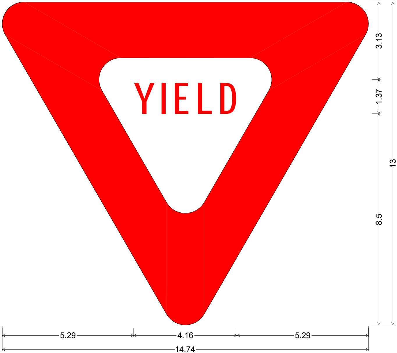
R1-2 (for use on R1-5); 16.02" corner to corner 0.88" Radius, 2.25" Border, Red on White; "YIELD" C;
