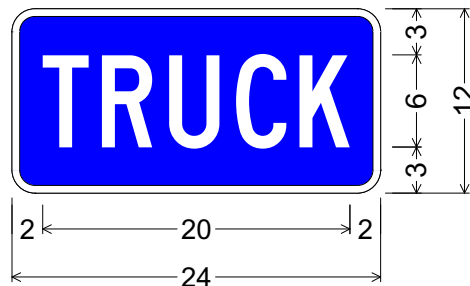
M4-4(24x12-STD)CLR; 1.50" Radius, 0.50" Border, White on Blue; "TRUCK" C 85% spacing;
