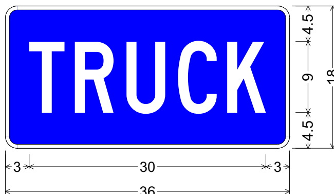
M4-4(36x18-FWY)CLR; 1.50" Radius, 0.50" Border, White on Blue; "TRUCK" C 85% spacing;
