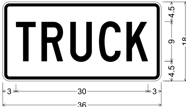
M4-4(36x18-FWY)WHT; 1.50" Radius, 0.63" Border, 0.38" Indent, Black on White; "TRUCK" C 85% spacing;
