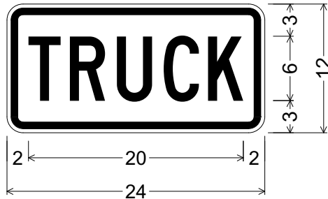
M4-4(24x12-STD)WHT; 1.50" Radius, 0.63" Border, 0.38" Indent, Black on White; "TRUCK" C 85% spacing;
