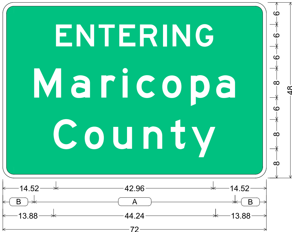
I3-102-FWY(Maricopa); 3.00" Radius, 1.00" Border, White on Green; "ENTERING" E; "Maricopa" E; "County" E;
