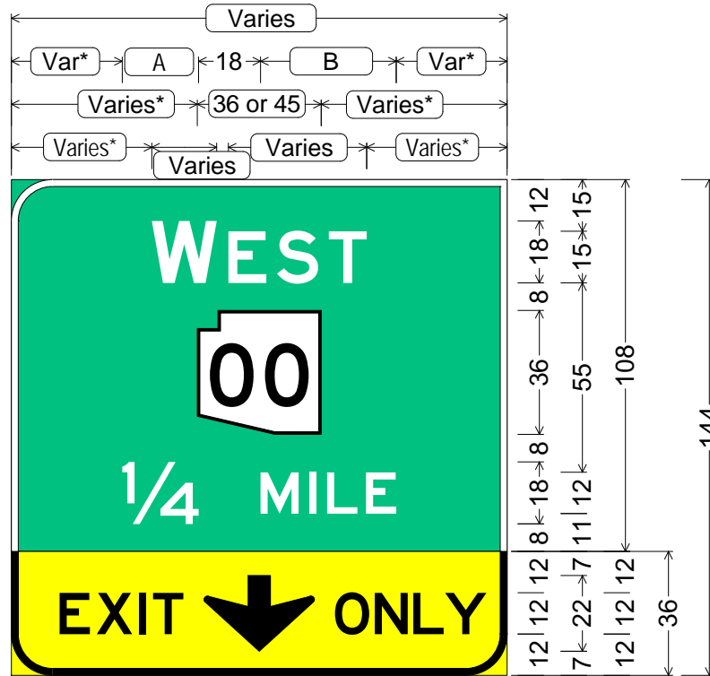
Var 36 6 32 6 44 Var E6-101edx (freeway - 36" shield)
