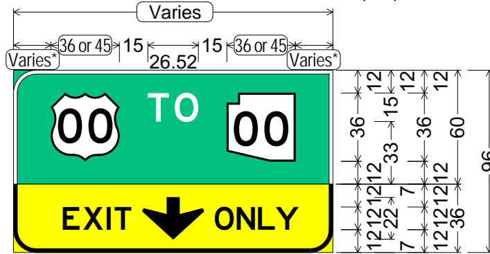
E6-101ex (freeway - 36" shield)
