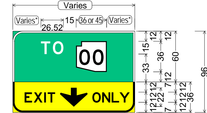
Varies ; 36 6 32 6 44 ; Varies E6-101ex (freeway - 36" shield)
