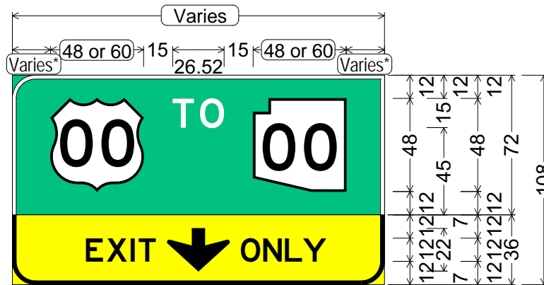
E6-101ex (freeway - 48" shield option)
