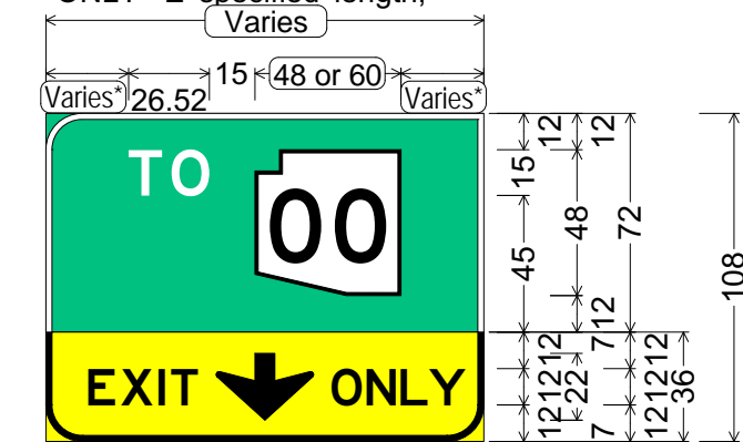
Varies ; 36 6 32 6 44 ; Varies E6-101ex (freeway - 48" shield option)
