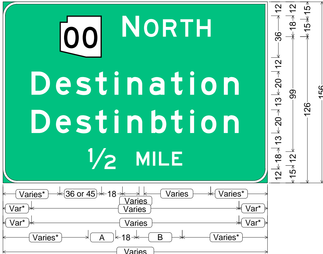
E1-101b (freeway); 12.00" Radius, 2.00" Border, White on Green; State Highway 00 M1-5c; "NORTH" E; "Destination" E; "Destinbtion" E; "1/2" E; "MILE" E;
