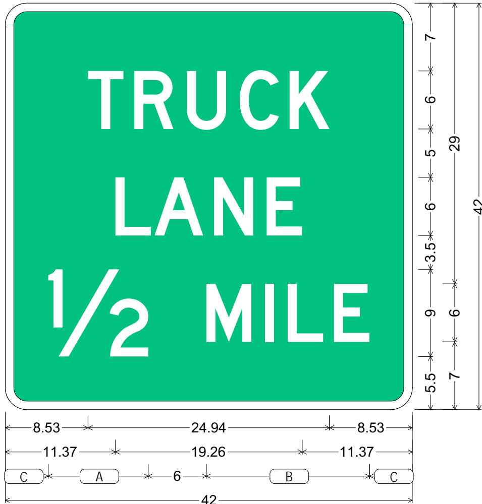
D17-2; 2.25" Radius, 0.88" Border, White on Green; "TRUCK" D; "LANE" D; "1/2" D; "MILE" D;
