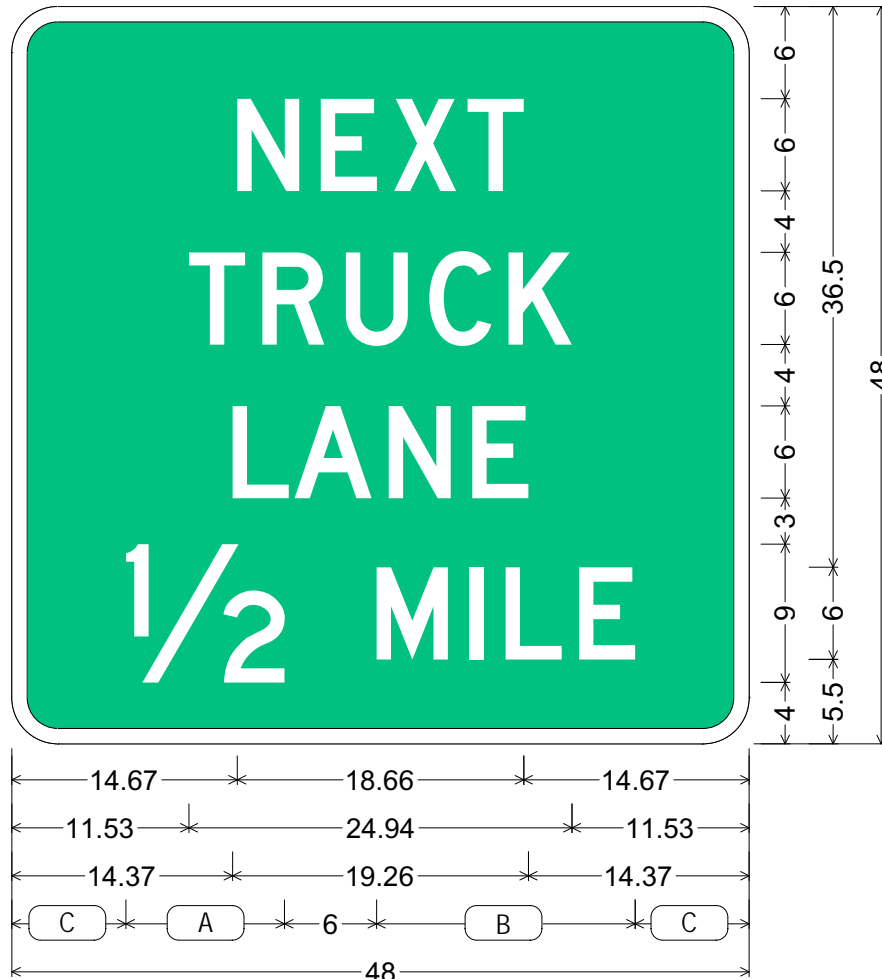
D17-1; 3.00" Radius, 1.00" Border, White on Green; "NEXT" D; "TRUCK" D; "LANE" D; "1/2" D; "MILE" D;
