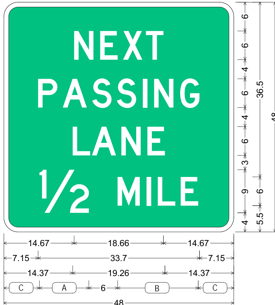
D17-1; 3.00" Radius, 1.00" Border, White on Green; "NEXT" D; "PASSING" D; "LANE" D; "1/2" D; "MILE" D;
