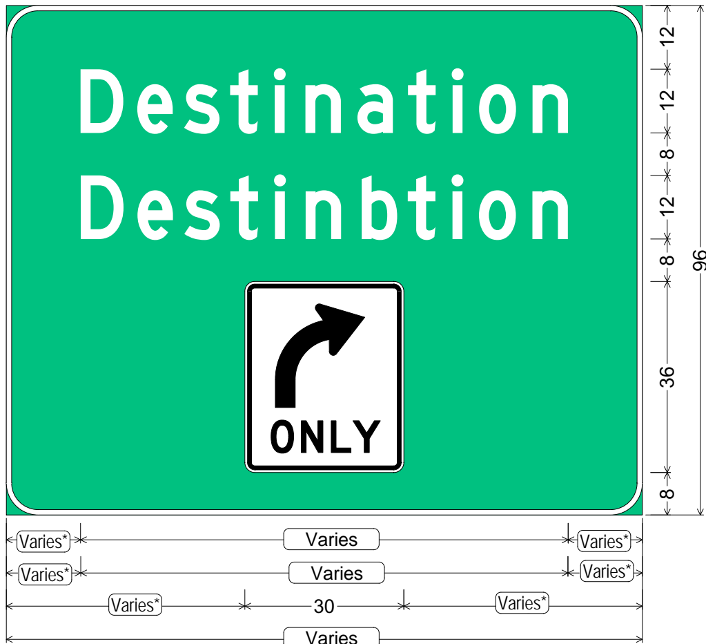
D15-101 (1 lane); 6.00" Radius, 1.00" Border, White on Green; "Destination" D; "Destinbtion" D; R3-5 or R3-5a - 30" x 36";
