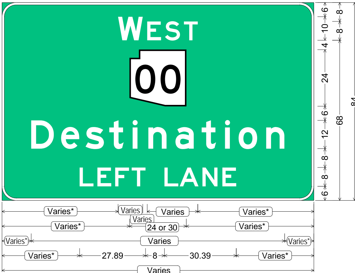
D1-107c (overhead); 6.00" Radius, 1.00" Border, White on Green; "WEST" E; State Highway 00 M1-5c; "Destination" E; "LEFT LANE" E;
