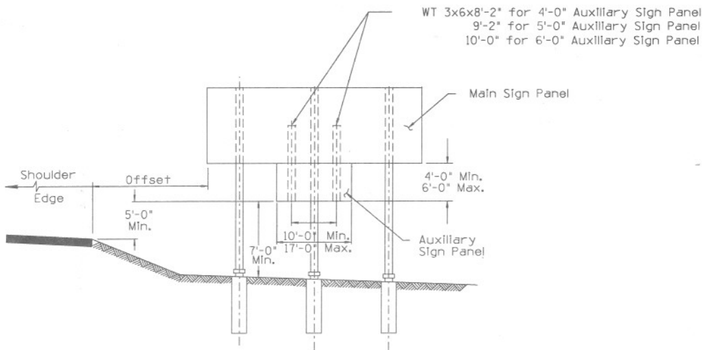
TWO POSTS SIGN Post Spacing greater than Width of Auxiliary Signs Minus 1'-0" & THREE POSTS SIGN
