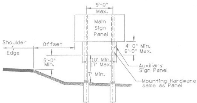
TWO POSTS SIGN Post Spacing Less than Width of Auxiliary Signs Minus 1'-0"
