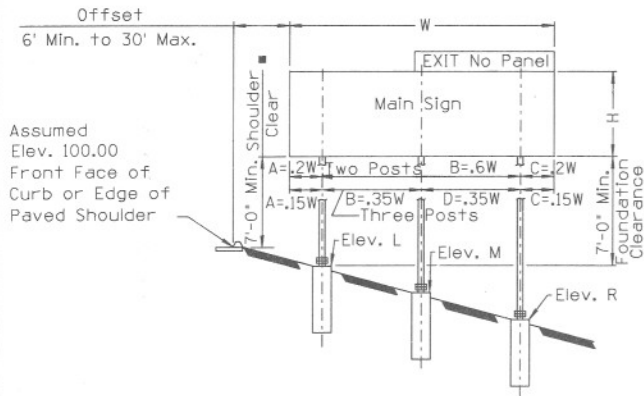
GUIDE SIGN INSTALLED ON SHOULDER
