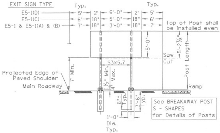
TYPICAL EXIT GORE SIGN
