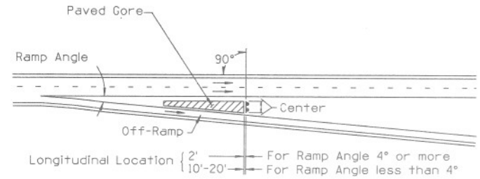
EXIT GORE SIGN LOCATION
