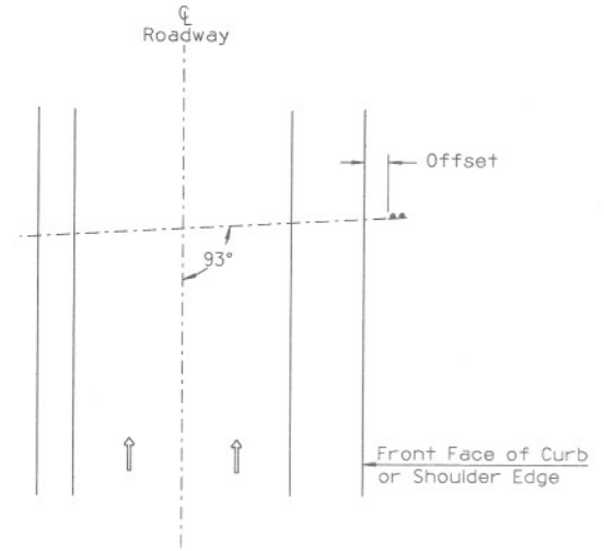
TYPICAL SIGN INSTALLATION ON SHOULDER
