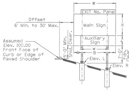
GUIDE SIGN WITH AUXILIARY SIGN INSTALLED ON SHOULDER
