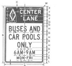
R3-11 * Reduce spacing 25% * Optically locate symbol B top legend
