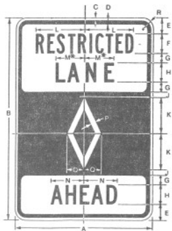
R3-10 * Increase spacing 100%
