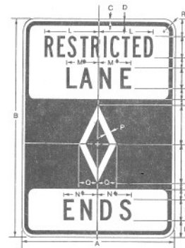
R3-12 * Increase spacing 100%
