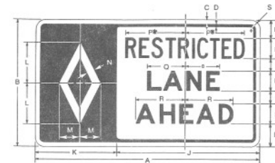
R3-13 * Reduce spacing 50%
