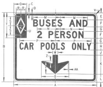
R3-15 * Reduce spacing 50%
