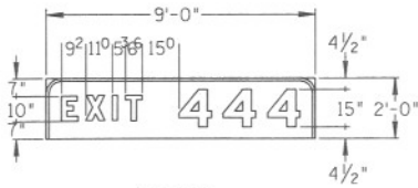
Exit Numbering Panel Three Digit
