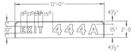
Exit Numbering Panel Four Digit
