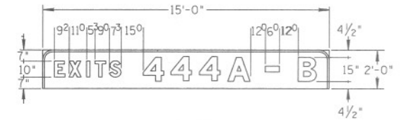
Exit Numbering Panel Five Digit
