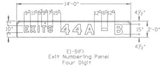
Exit Numbering Panel to be used with Existing Sign E5-1
