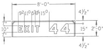
Exit Numbering Panel Two Digit
