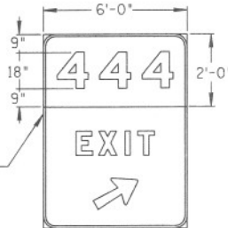
Exit Numbering Panel to be used with Existing Sign E5-1
