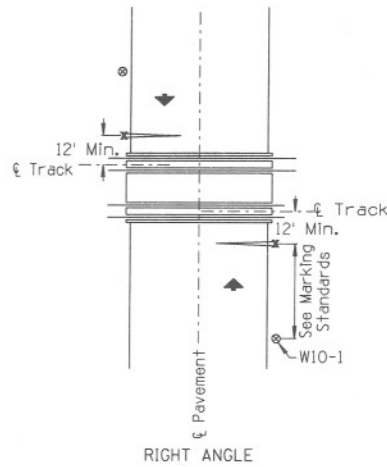
TYPICAL LOCATION PLANS FOR FLASHING LIGHT SIGNALS AND AUTOMATIC GATES
