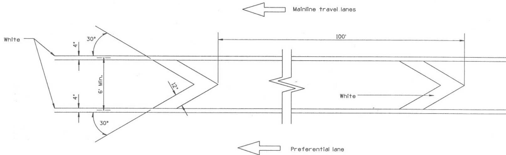
PREFERENTIAL LANE BUFFER DETAIL
