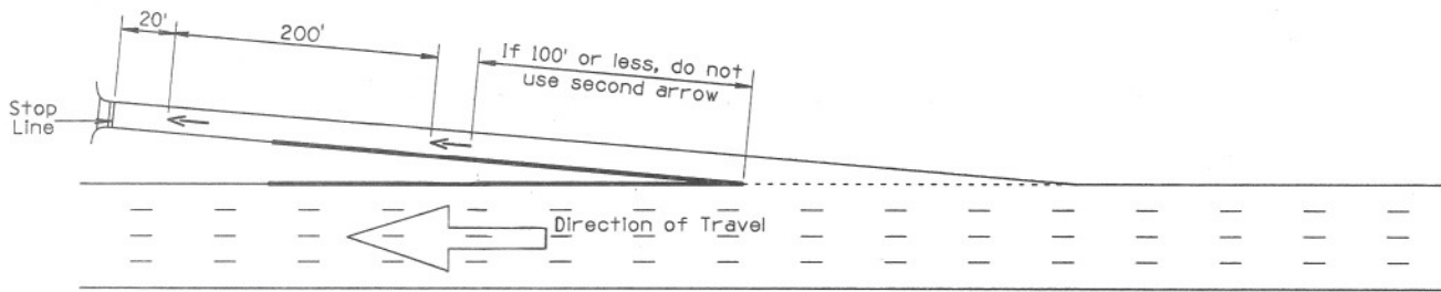
ONE LANE TERMINAL
