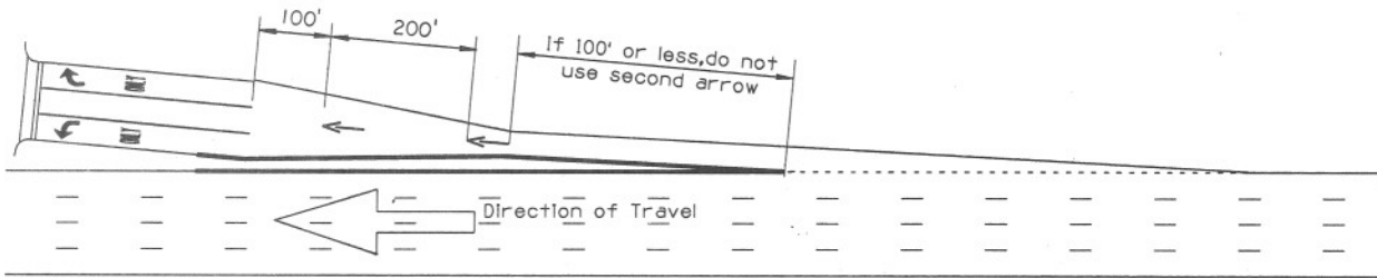
THREE LANE TERMINAL WITH ONE EXIT LANE
