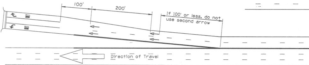
THREE LANE TERMINAL WITH TWO EXIT LANES
