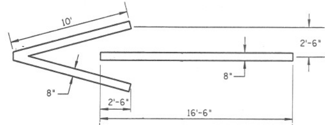
FREEWAY, EXPRESSWAY AND RAMP PAVEMENT ARROW
