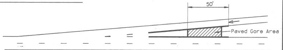
OPTIONAL ON-RAMP APPLICATION
