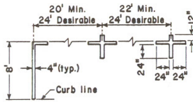
STANDARD PARALLEL PARKING DETAIL
