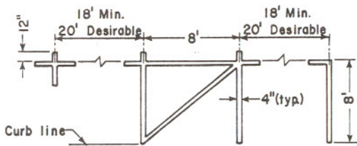
TANDEM PARALLEL PARKING DETAIL
