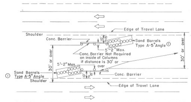
DOUBLE PIER OR COLUMN
