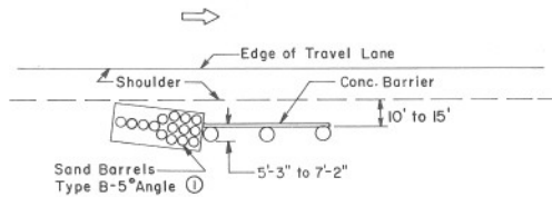
TRAFFIC ON ONE SIDE ONLY
