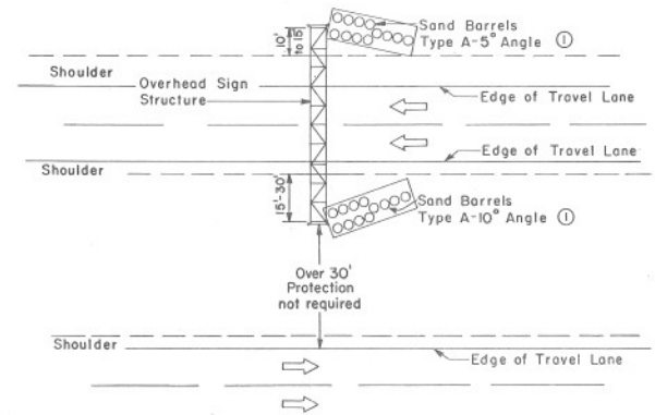
OVERHEAD SIGN STRUCTURE
