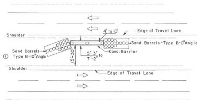
OFFSET SINGLE PIER OR COLUMN
