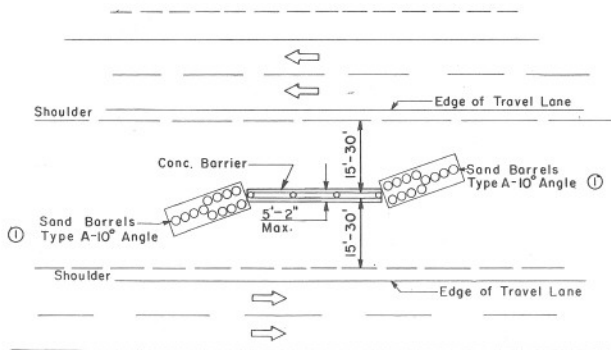
SINGLE PIER OR COLUMN
