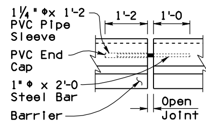
JOINT BAR DETAIL
