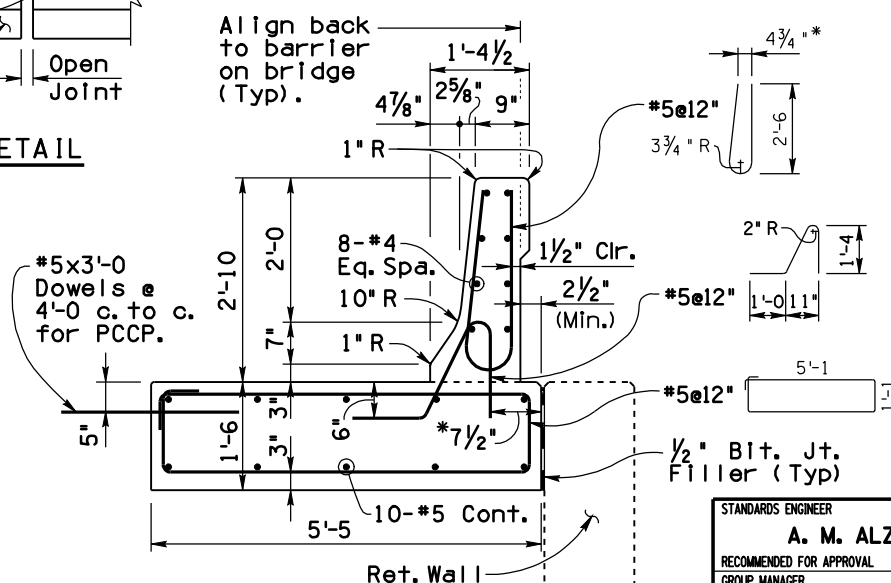
SECTION Continuous Barrier With Footing
