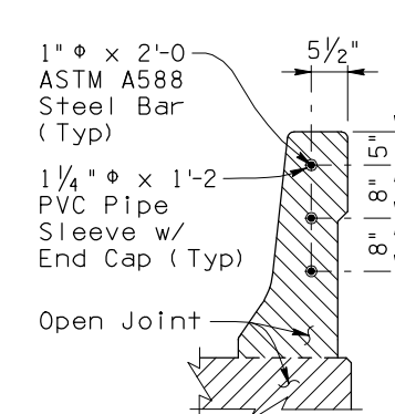
OPEN JOINT DETAIL At Expansion Joints
