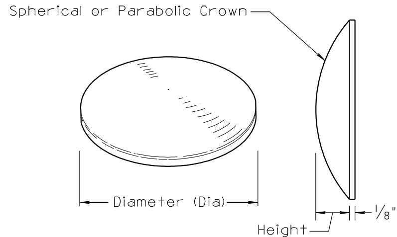
TYPES A, AY AND AB (Types B and BY (Not Shown))
