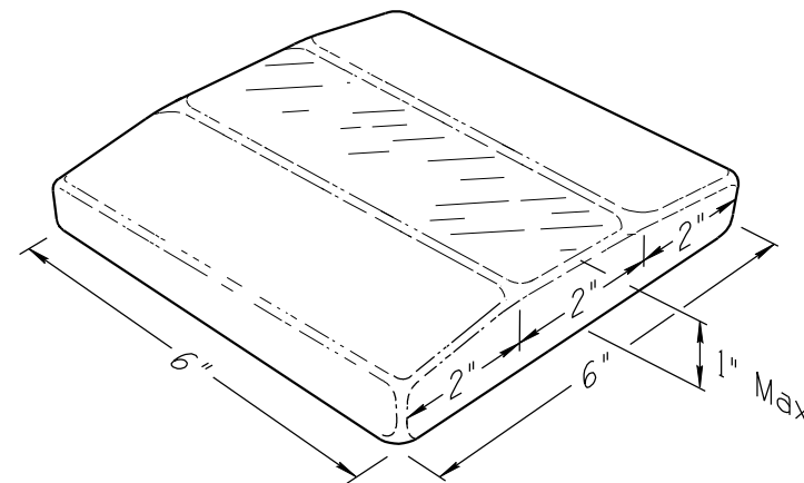
TYPES O AND OY JIGGLE BAR
