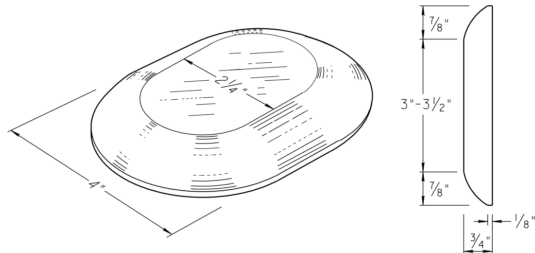
TYPES Q AND QY OVAL
