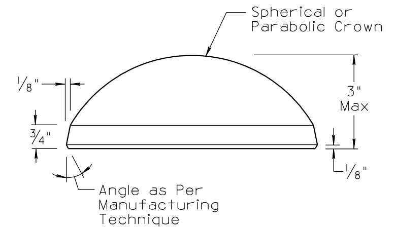
TYPES M AND MY, (Large Channel Marker)
