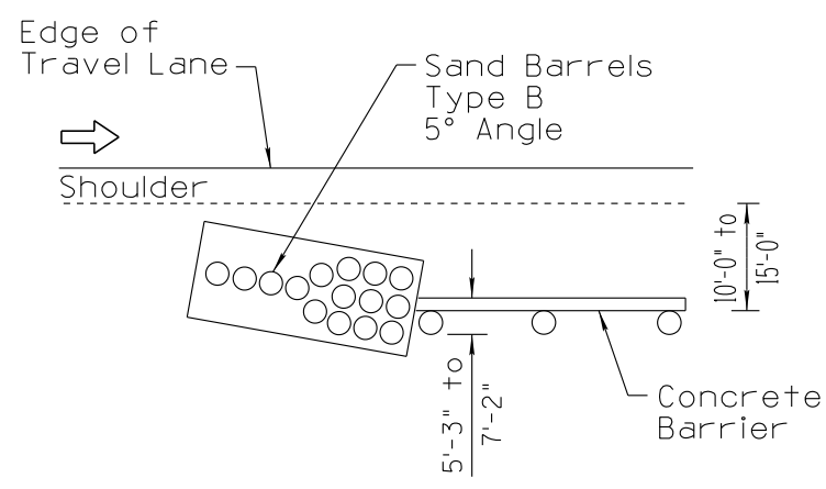
TRAFFIC ON ONE SIDE ONLY
