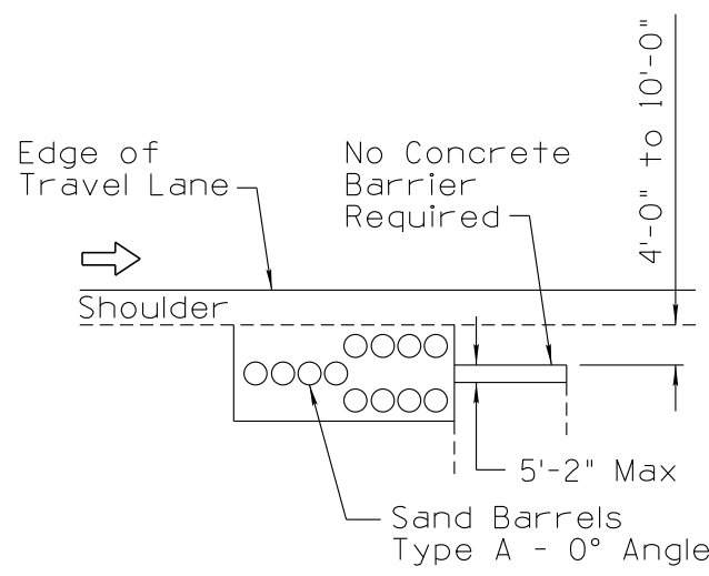
SOLID PIER OR ABUTMENT
