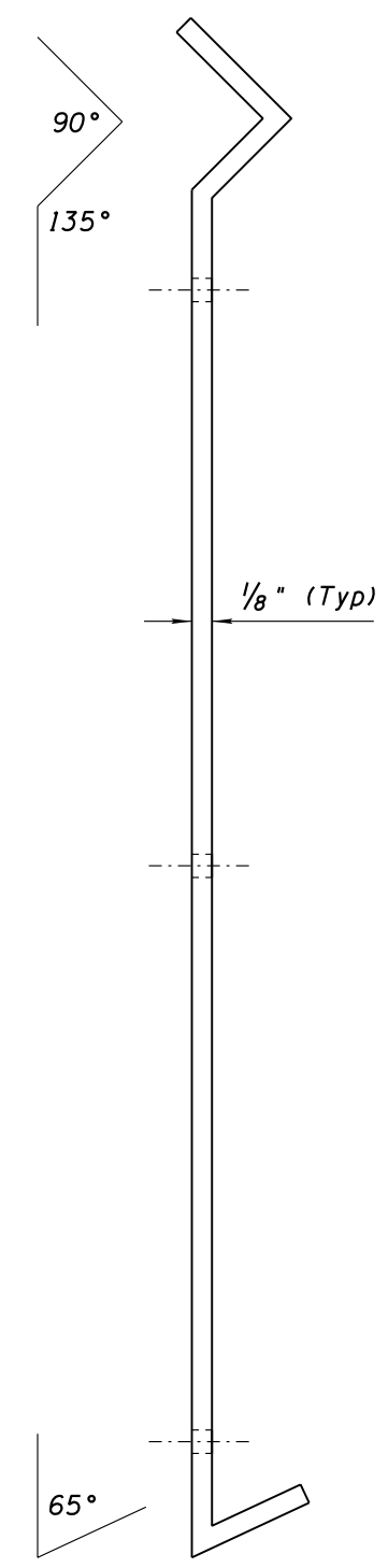
SIDE PANEL LEFT SIDE VIEW
