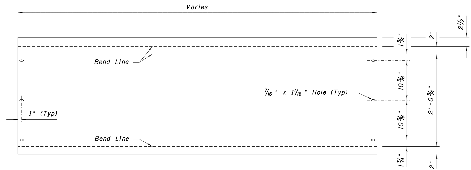
SIDE PANEL UNFOLDED
