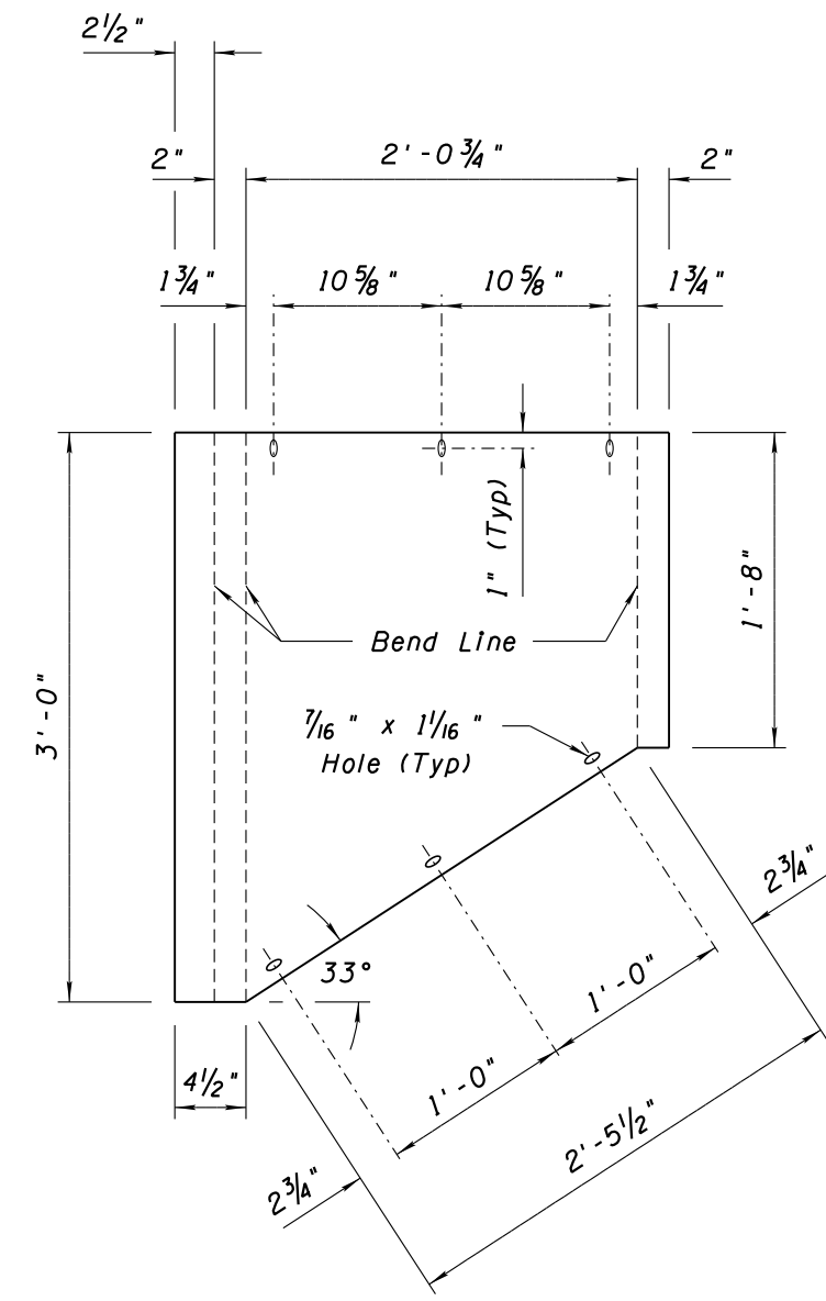
LEFT RIDER SIDE PANEL UNFOLDED
