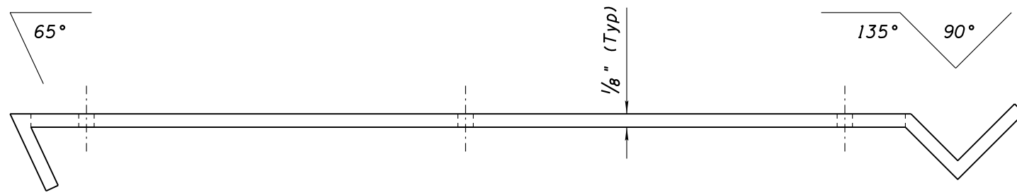
RIGHT RIDER SIDE PANEL TOP VIEW
