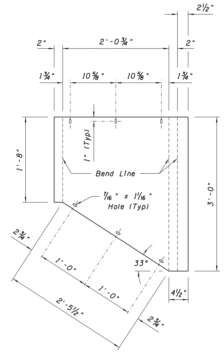
RIGHT RIDER SIDE PANEL UNFOLDED
