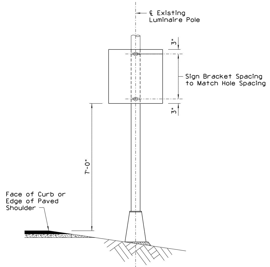
TYPICAL INSTALLATION OF SIGN ON POLE
