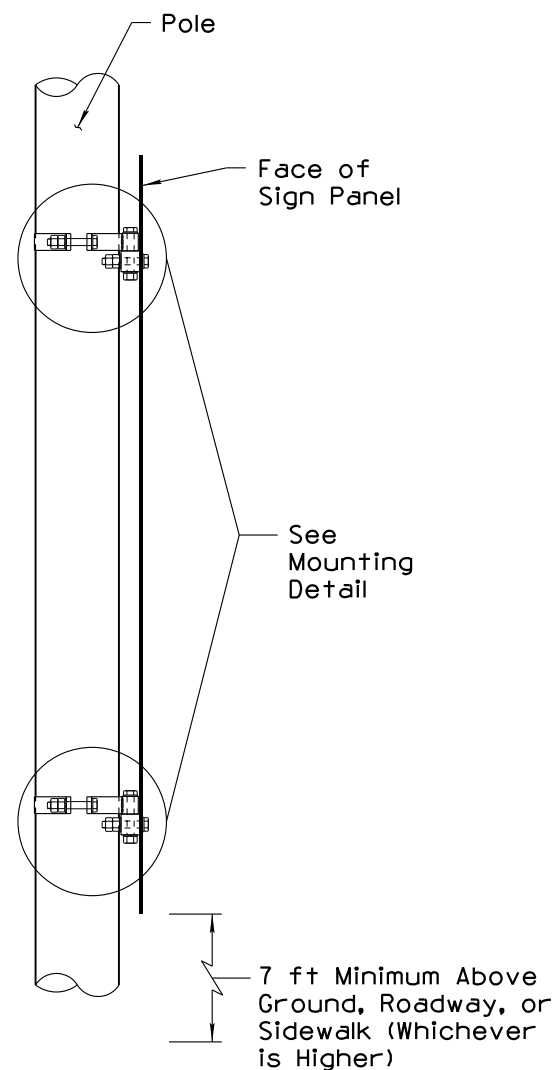
SIDE VIEW
