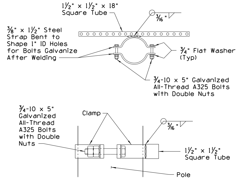
CLAMP DETAIL
