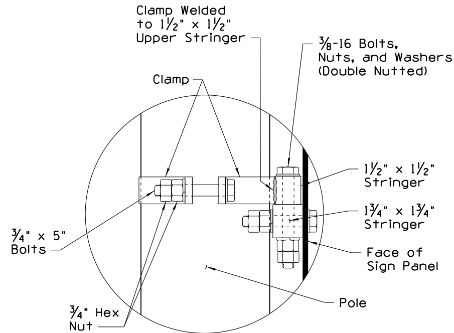
MOUNTING DETAIL
