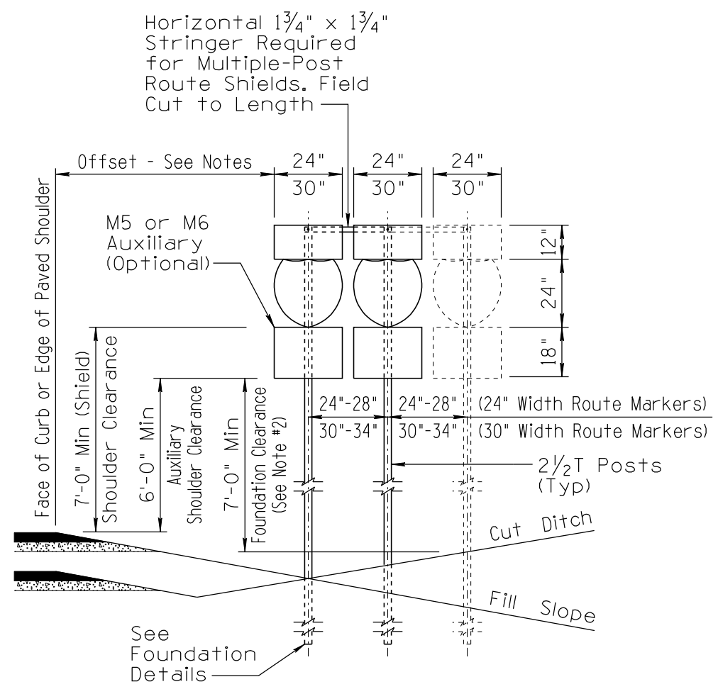
MULTIPLE ROUTE MARKER Conventional Road (Including Freeway Ramp or Crossroad) 24 and 30 Inch Width Route Markers
