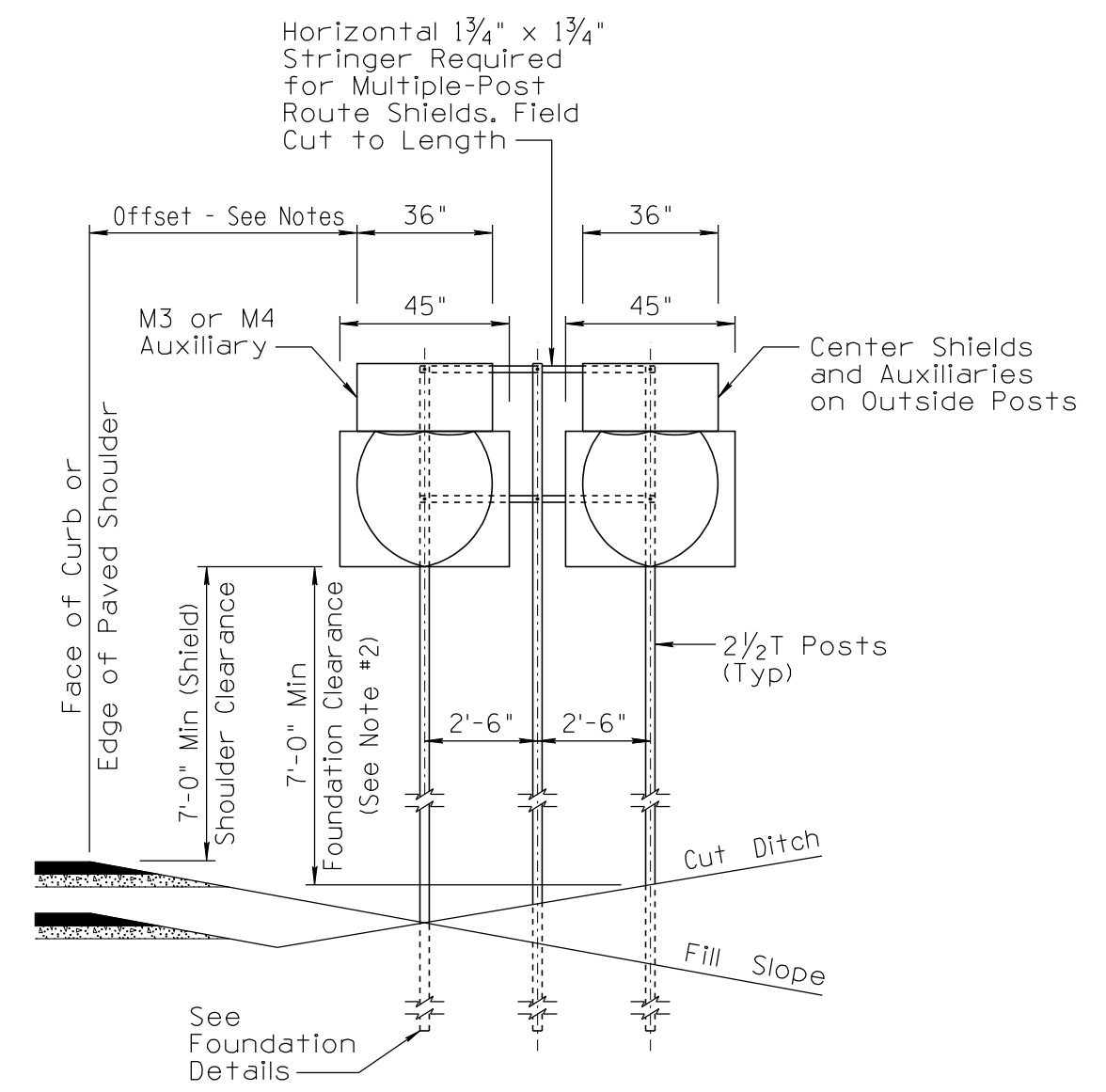
MULTIPLE ROUTE MARKER Freeway or Expressway Mainline 36 and 45 Inch Width Route Markers
