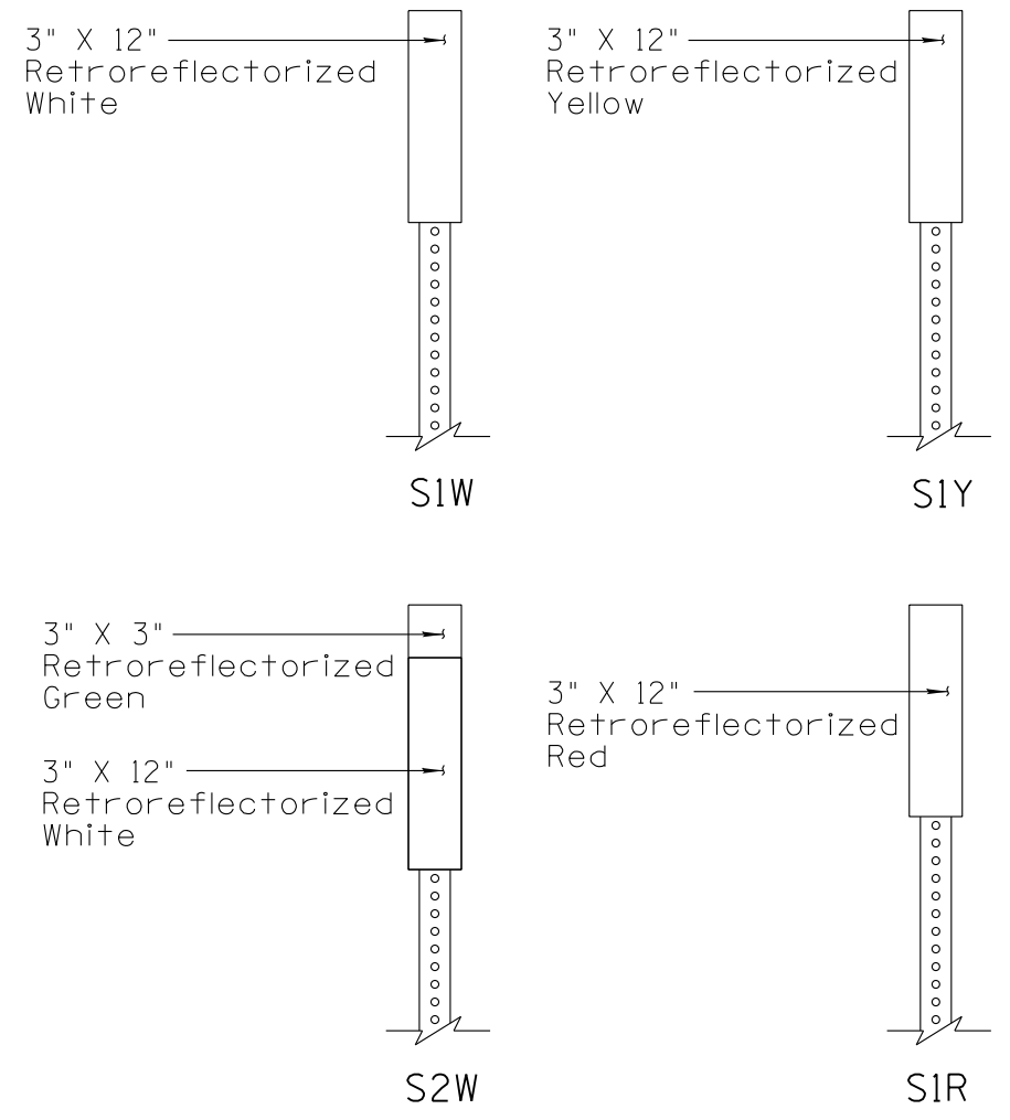
STEEL POST DELINEATOR FACES
