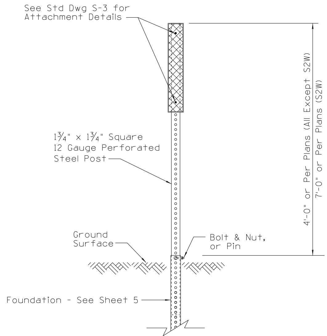
SQUARE STEEL POST DELINEATORS ASSEMBLY
