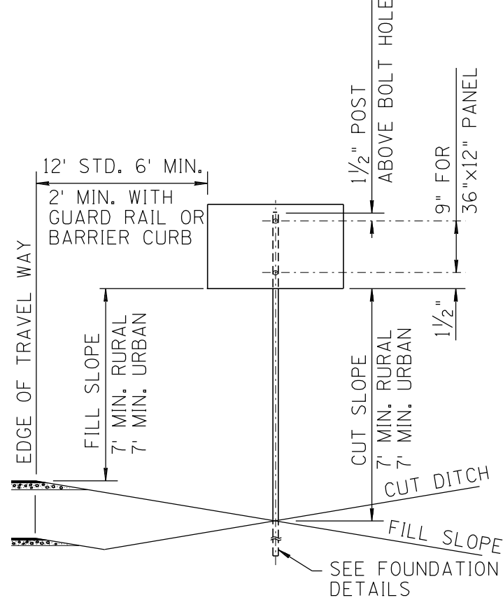
REGULATORY SIGN SINGLE POST
