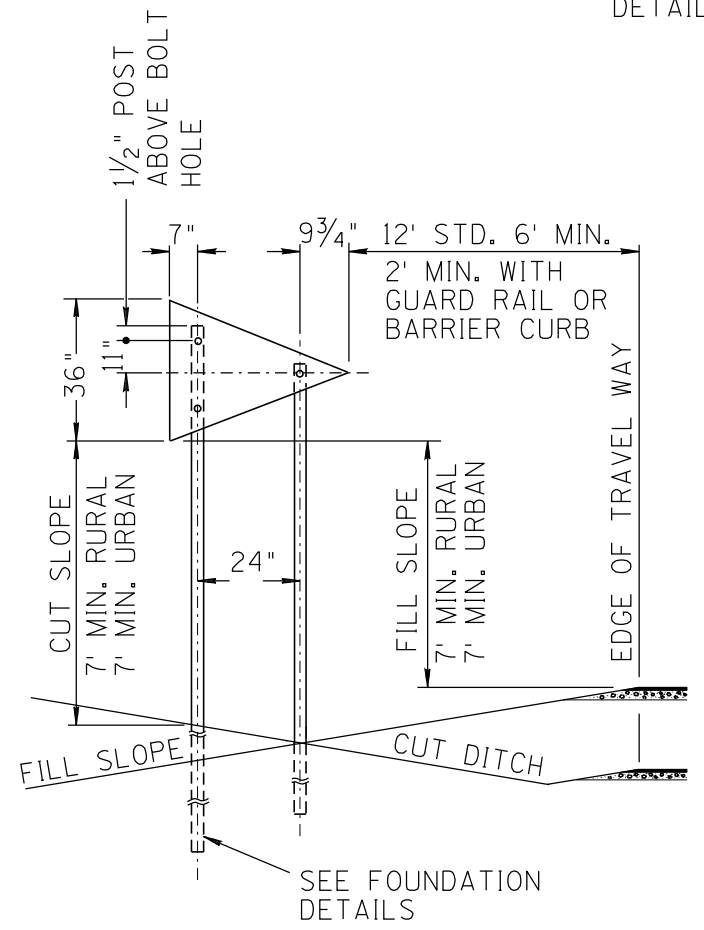
NO PASSING PENNANT
