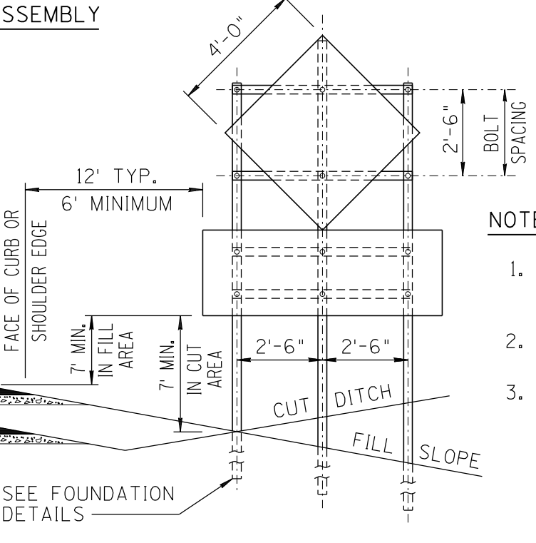
WARNING SIGN WITH LARGE AUXILIARY PLAQUE (8 SQUARE FEET OR MORE)
