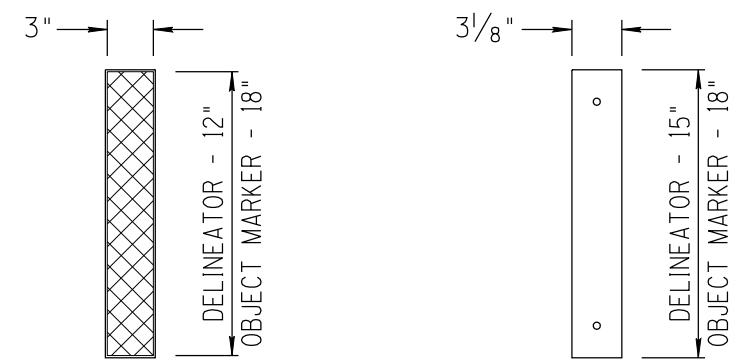
REFLECTOR REFLECTIVE PANEL (PRE-DRILLED/PUNCHED) (OR AS DETAILED ON OTHER PLANS)
