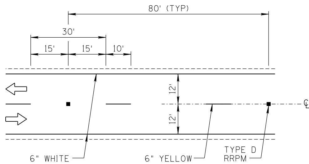
TWO-WAY PASSING ZONE
