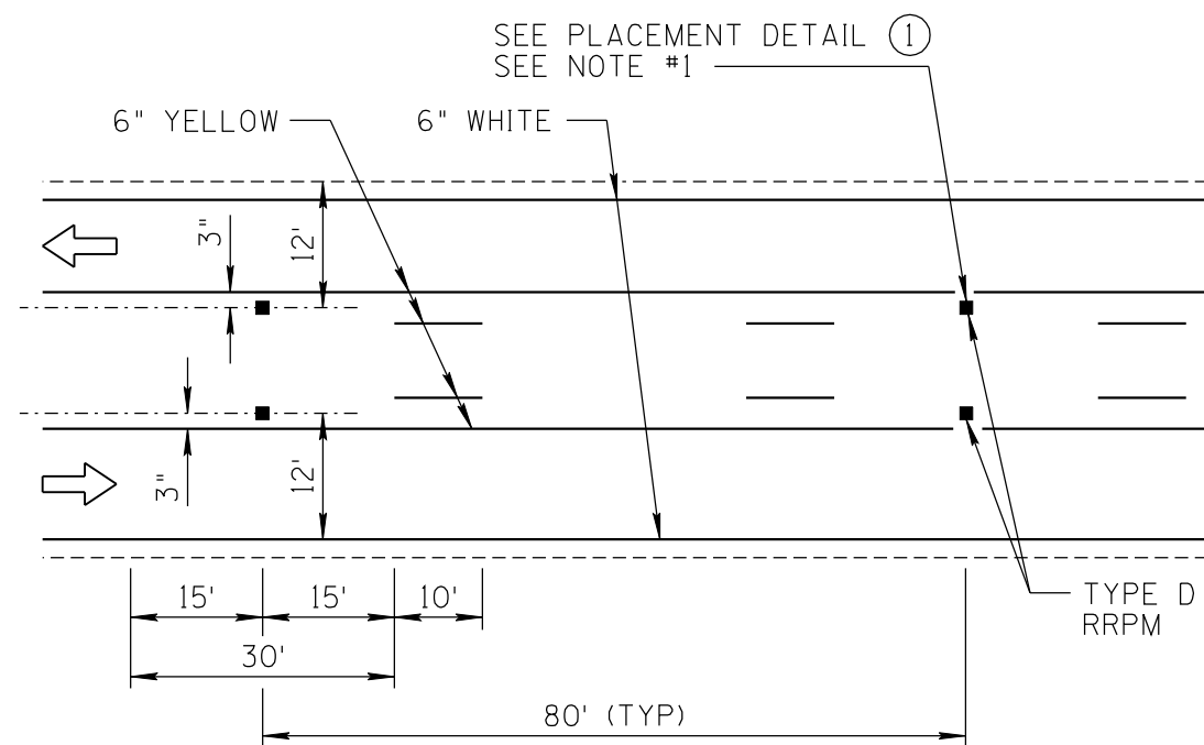
TWO-WAY LEFT-TURN LANE
