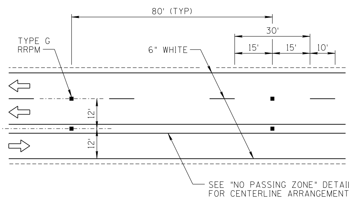
PASSING/CLIMBING LANE
