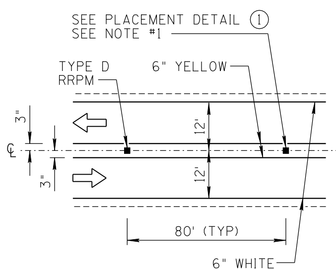
NO PASSING ZONE
