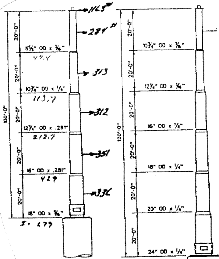
ELEVATION 100' POLE HM100Z
