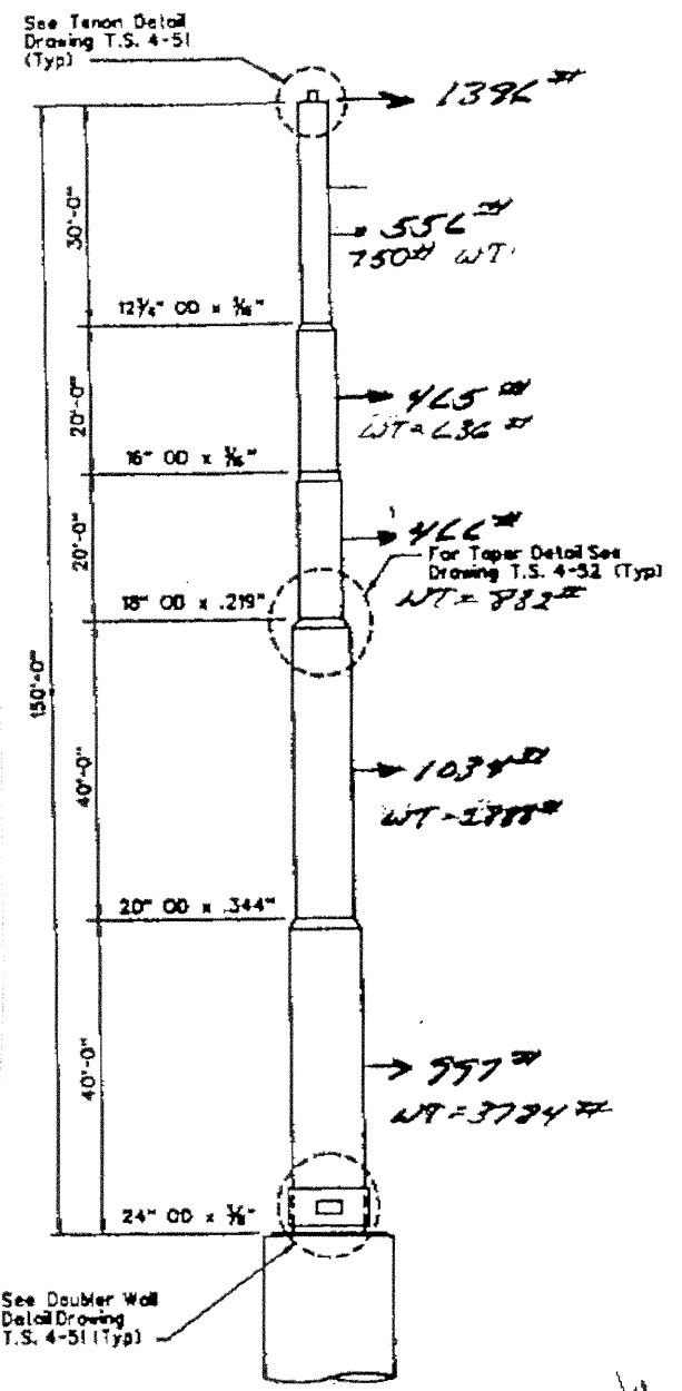
ELEVATION 150' POLE HM150Z
