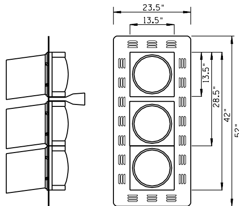
TYPE "F" (WITH ELEVATOR PLUMBIZER)
