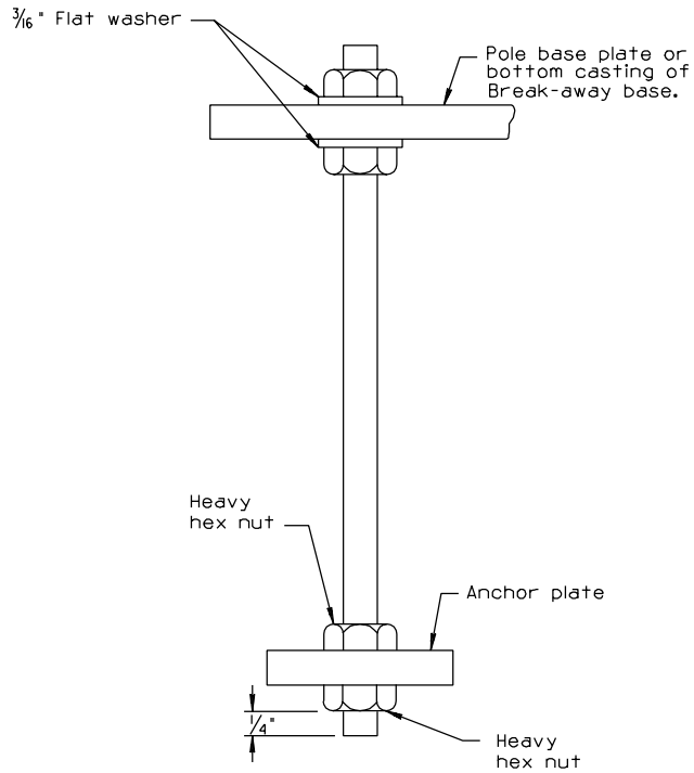
ANCHOR BOLT DETAIL
