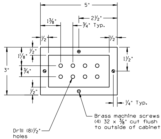
VENTILATION DETAIL
