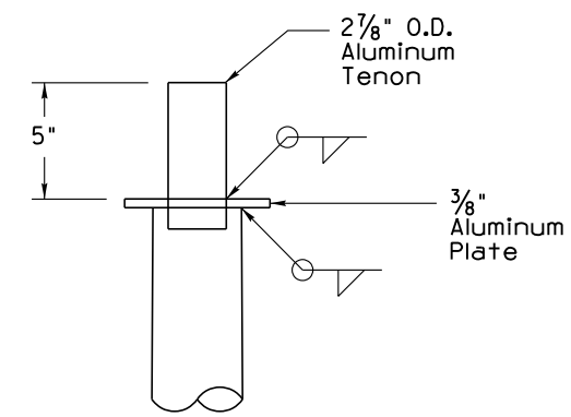
POLE TOP DETAIL
