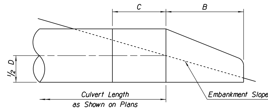
RIGHT-ANGLE CULVERT
