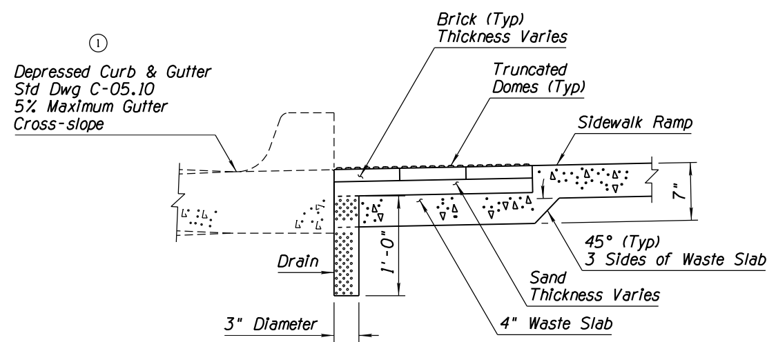
DETECTABLE WARNING STRIP BRICK OPTION
