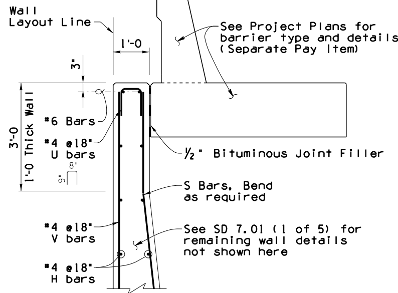
TYPICAL WALL DETAILS (Case IV)
